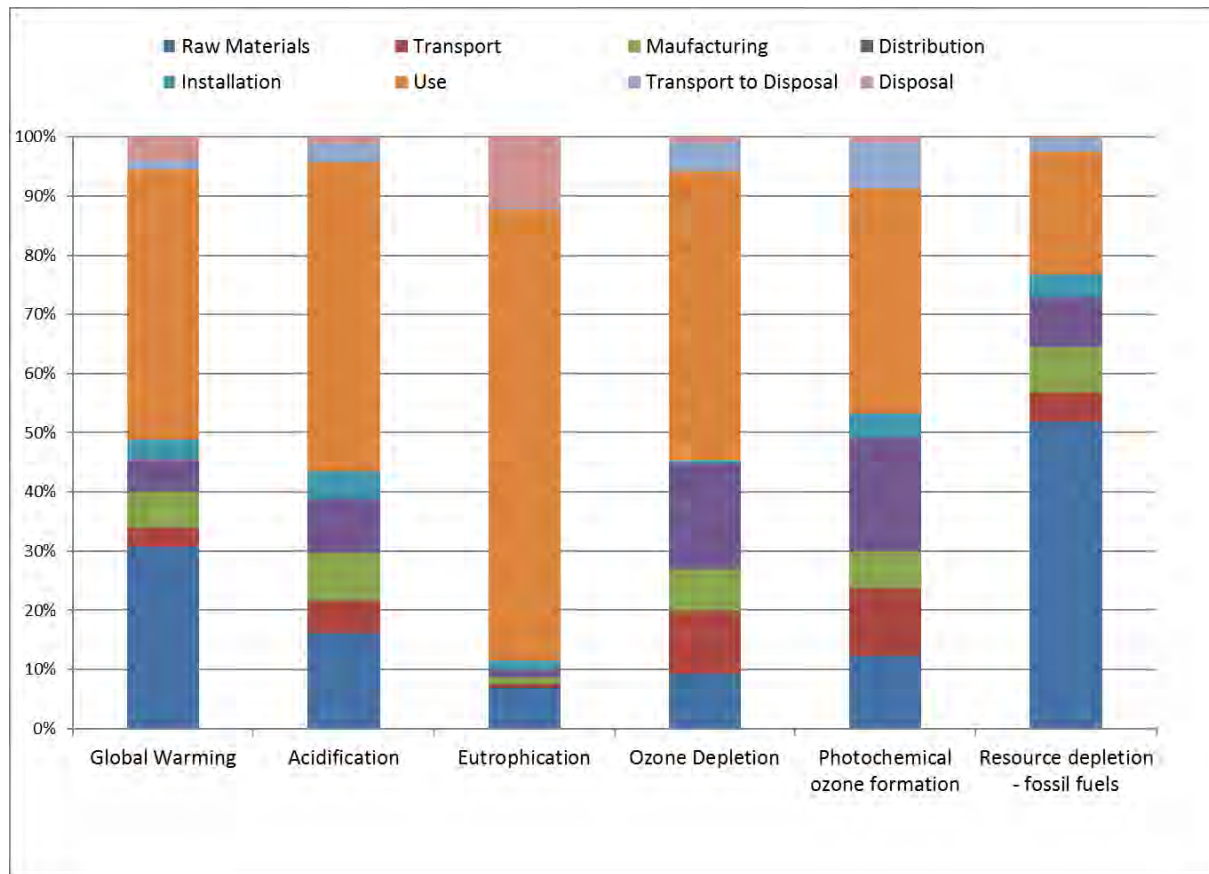
Figure 3. Contribution analysis for the AFIRMA™ II Hardback Tile (Continuous Dyed) product system – TRACI v2.1
