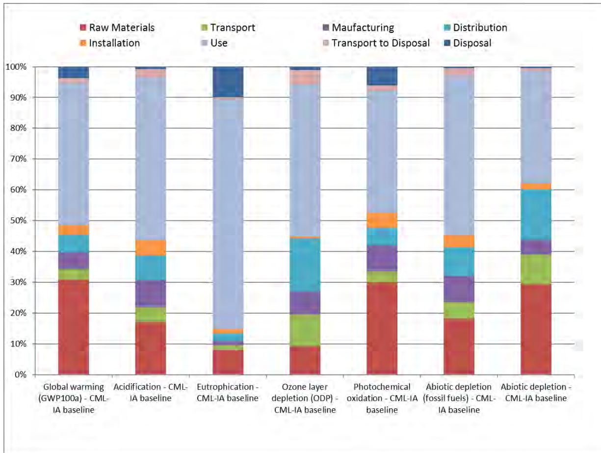
Figure 2. Contribution analysis for the AFIRMA™ II Hardback Tile (Continuous Dyed) product system – CML-IA
